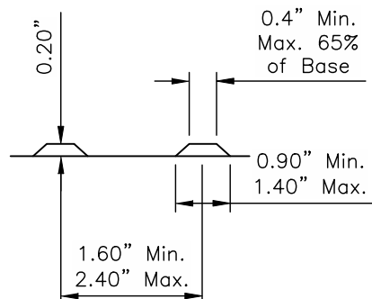
SECTION "C-C" Dome Tolerances
