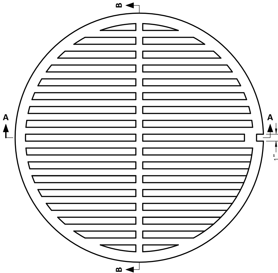
PLAN VIEW
