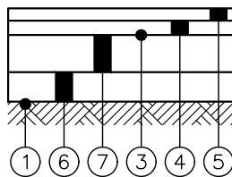
TYPE 2B ASPHALT PAVEMENT
