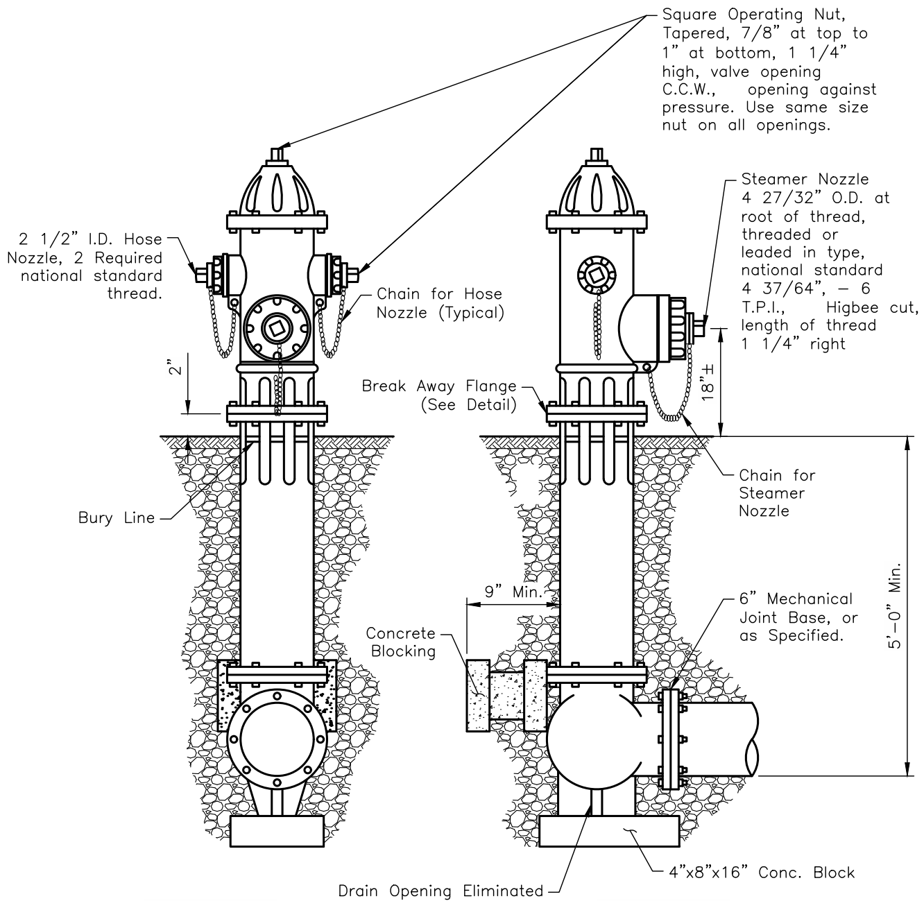
FRONT VIEW
