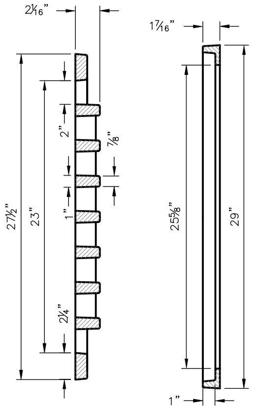
GRATE SECTION B-B FRAME SECTION B-B
