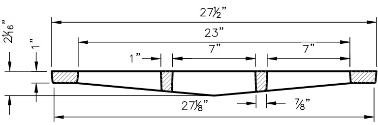
GRATE SECTION A-A
