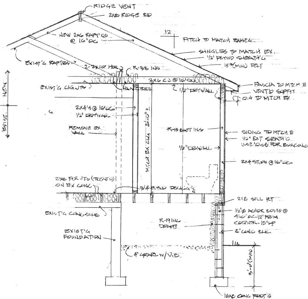
BUILDING SECTION SCALE: 3/8" = 1'-0"
