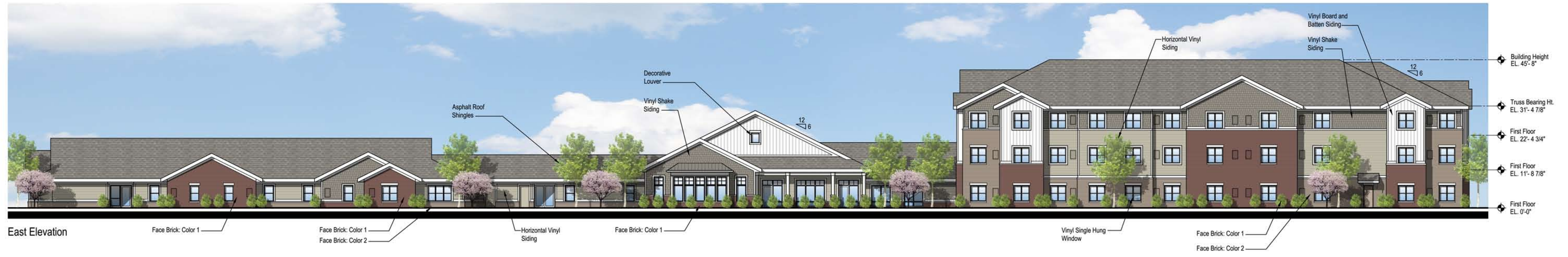
North Elevation (Main Entry)
